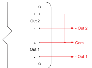
Outputs > 500Vdc
